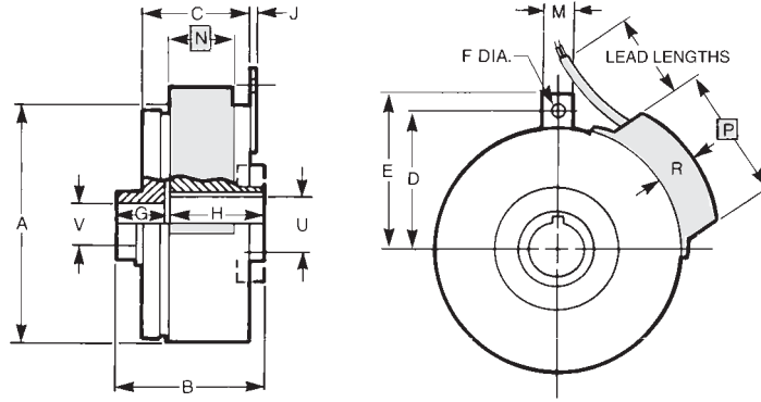
Standard DC Clutch
